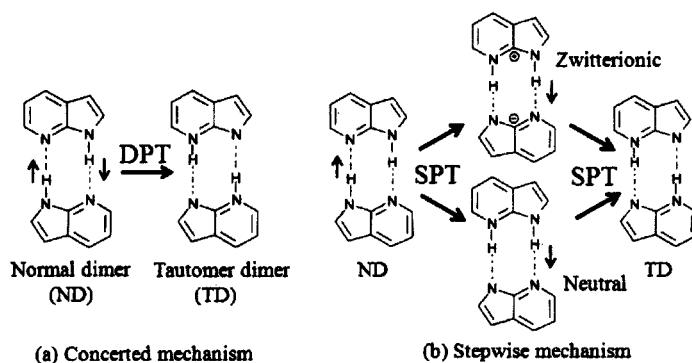
Fig. 1. Concerted mechanism vs. stepwise mechanism for ESDPT in 7AI dimer.
