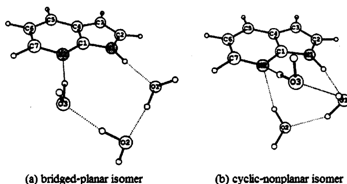
Fig. 2. Equilibrium structures of 7\text{Al}(\text{H}_2\text{O})_3 in the excited
